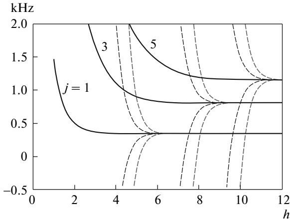
Fig. 2. The energies of the gravitational quantum states \epsilon_j(h) for j = 1, 3, 5 as functions of the waveguide width h (solid lines). The dashed lines show the line broadening \epsilon_j \pm 1/2\tau_j in kHz. The roughness is exponential in one (black dashed lines) or two (grey dashed lines) dimensions with \eta = r = 1 . Scaling (31) allows recalculating the broadening for different \eta and r .
