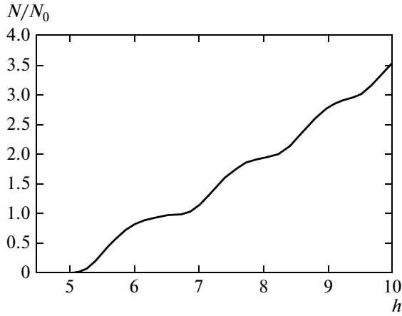
Fig. 3. The exit neutron count N(h)/N_0 , Eq. (26), as a function of the spacing between the mirrors. Calculations for the new sapphire mirror with isotropic exponential roughness r = 0.65 , \eta = 1.02 .
