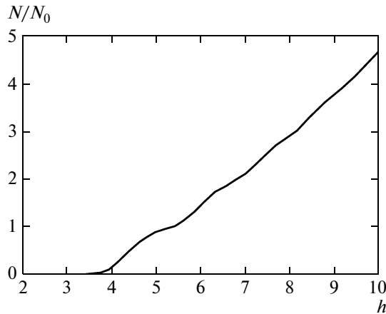
Fig. 5. The exit neutron count N(h)/N_0 , Eq. (26), for the Ising mirror similar to the one in Fig. 2. The roughness amplitude is \eta = 0.4 and the correlation radius is r = 2 . The steps can be made more pronounced by increasing \eta .
