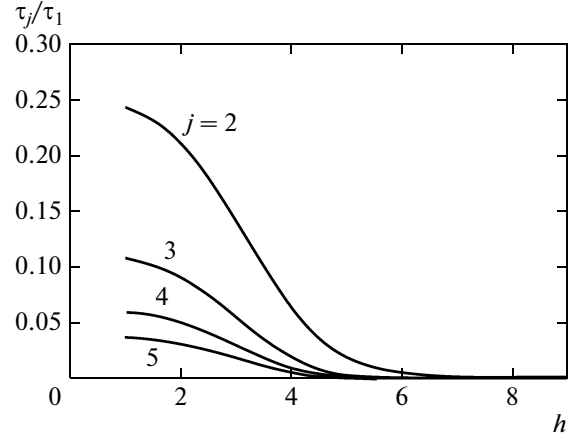
Fig. 1. The ratios \tau_j(h)/\tau_1(h) , Eq. (18), for the lowest quantum levels j = 2, 3, 4, 5 as functions of the slit width h . The curves are marked by the values of j . These functions are the same for 1D and 2D roughness and do not depend on the roughness parameters.
