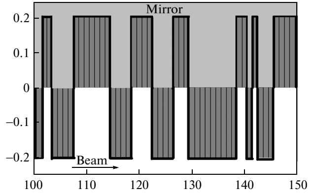
Fig. 4. A fragment of the rough upper mirror based on Monte Carlo simulations for the 1D Ising model (the Ising mirror). The thick black line is the surface profile and dark bars are “Ising spins.” Mirror material (sapphire) is above the thick black line (all dark and light filled areas). The amplitude of roughness is \eta = 0.2 , the correlation radius is r = 2 , and \Phi_1 \approx 43.5 . Both axes are in units of l_0 = \hbar^{2/3}(2m^2g)^{-1/3} \approx 5.871 \mu\text{m} and the vertical scale is about 100 times smaller than the horizontal one. Changing the value of \eta can be done simply by rescaling the vertical axis.
